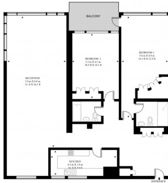
SIXTH FLOOR
